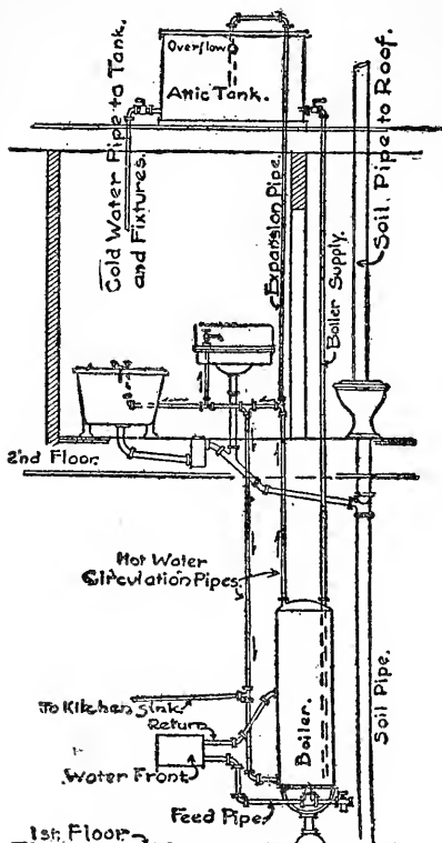
Hot-water circulation. (E. T. Wilson.)
