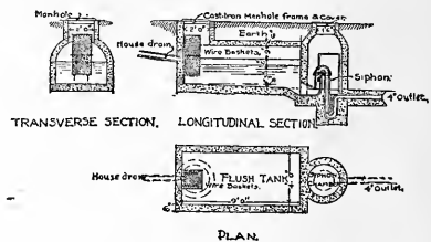
Simple flush tank. (E. T. Wilson.)
