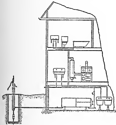
Water distribution by pneumatic tank system. Courtesy State Board of Health of Maine.
