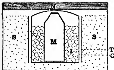
Vertical section of homemade milk refrigerator; S, sawdust; T, cylinder of tin or galvanized iron; C, can or pail, in which is placed the milk bottle M, surrounded by broken ice, I; N, newspapers nailed to lid of case. Courtesy Health Department of Chicago.
