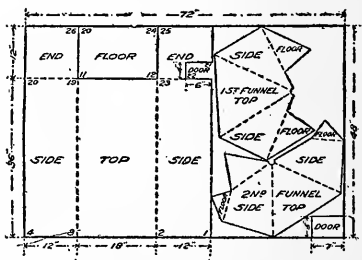
Diagram for cutting out the parts of a funnel trap 36 x 18 x 12 inches. (Ned Dearborn.)
