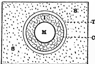
Horizontal section of homemade milk refrigerator; M, milk bottle; I, broken ice; C, can or pail for holding ice; T, tin or galvanized iron cylinder to prevent sawdust, S, from falling into space when can is removed for purpose of emptying water. Courtesy Health Department of Chicago.
