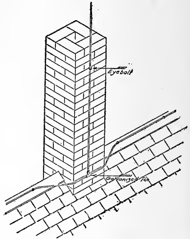
Showing method of running horizontal conductor around a chimney or cupola. (Alfred J. Henry.)
