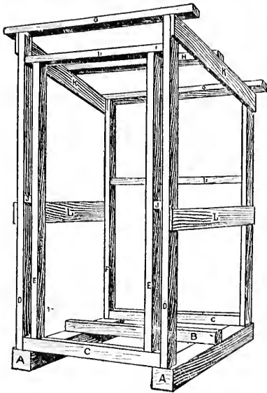
Framework of the sanitary privy.
