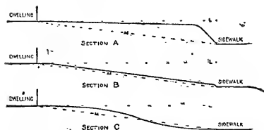
Cross sections of bad and good grading of small front yards. L indicates the level of the house foundation, and M a straight line from the top of the house foundation to the sidewalk level. Section A: Bad, with the rare exception of where a strictly formal treatment is admissible. Section B: Bad. Section C: Good. This curve may be short or long to accommodate the difference in height between the dwelling and sidewalk, and the distance between them. (L. C. Corbett.)
