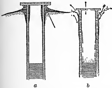
(a) Proper method of walling up and protecting private wells from surface drainage; (b) unprotected private well. ( Ritchie's Primer of Sanitation . Copyright, 1909, by World Book Company, Yonkers, New York.)
