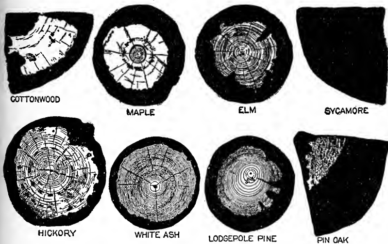
Sections of posts of various woods treated with creosote by the open-tank process. All the posts are drawn to the same scale, and are approximately 5 inches across. The black areas show the creosote penetration, which corresponds generally to the sapwood. (C. P. Willis.)
