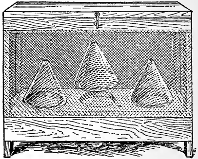
Box fly trap designed by C. F. Hodge.
