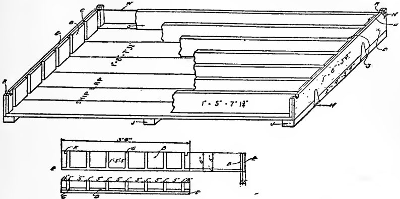
Gang mold for posts without taper. (Office of Public Roads.)
