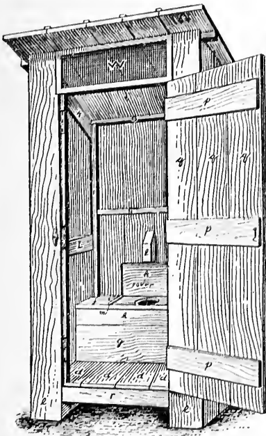
The sanitary privy. Front view.
