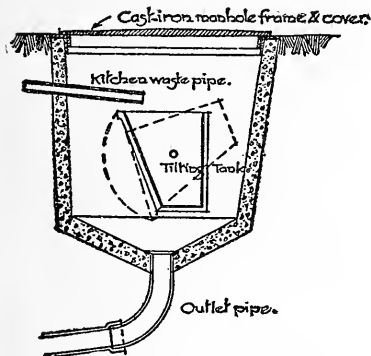
Tilting tank. (E. T. Wilson.)
