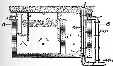
Section of septic tank. Courtesy State Board of Health of Maine.
