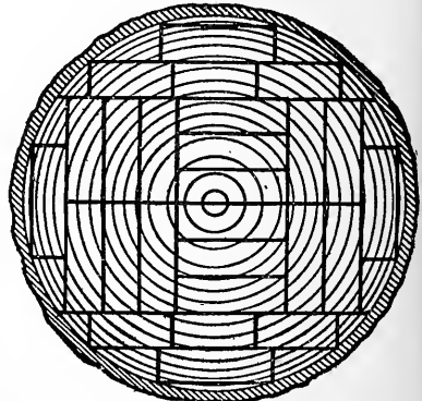
Method of cutting planks from logs. (C. L. Hill.)
