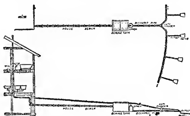
Details of a typical surface irrigation plant in plan and section. Courtesy State Board of Health of North Carolina.
