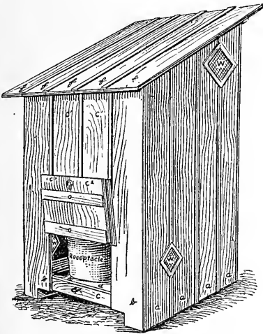
The sanitary privy. Rear and side view.
