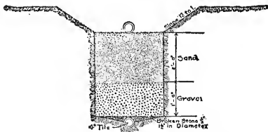
Section of filter bed. (E. T. Wilson.)
