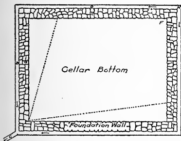
Method of draining cellar bottom. Courtesy State Board of Health of Maine.
