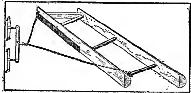
Perspective view of split-log drag. (D. Ward King.)
