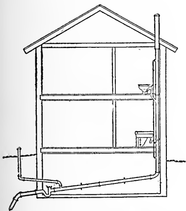
Plan of soil pipe for house sewage disposal system. Courtesy State Board of Health of Maine.
