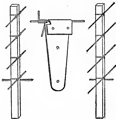
Methods of attaching fence wire to concrete posts. (Office of Public Roads.)
