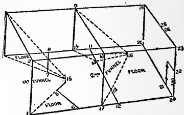
Outline of funnel trap. (Ned Dearborn.)
