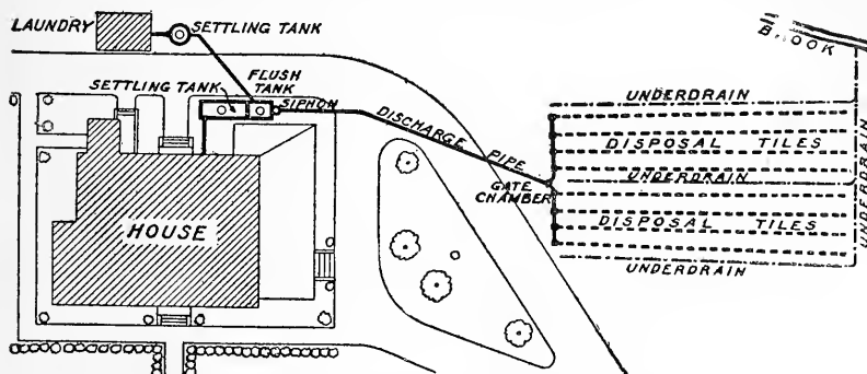
Rectangular tanks close to house. Separate settling tank for laundry building. Underdrains in disposal area to drain out underlying ground water and water from purified sewage in naturally wet or dense soil. Courtesy State Board of Health of North Carolina.
