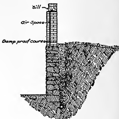
Method of draining cellar walls. Courtesy State Board of Health of Maine.
