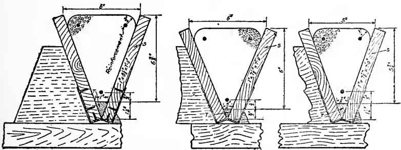
Molds for triangular posts. (Office of Public Roads.)
