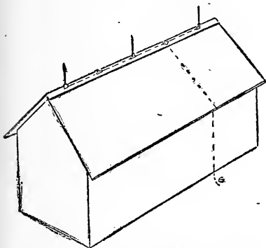
Method of placing lightning rods on a building having no cupola or chimney. Length of building, about 25 feet. (Alfred J. Henry.)
