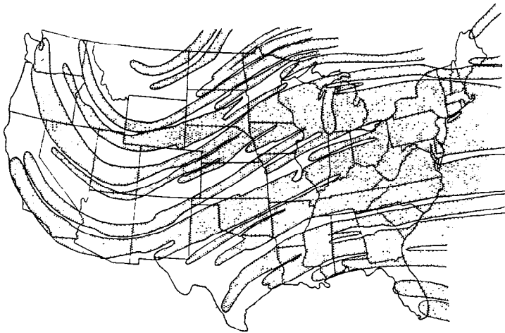
Figure 2.—Fallout areas at 24 hours after detonation
