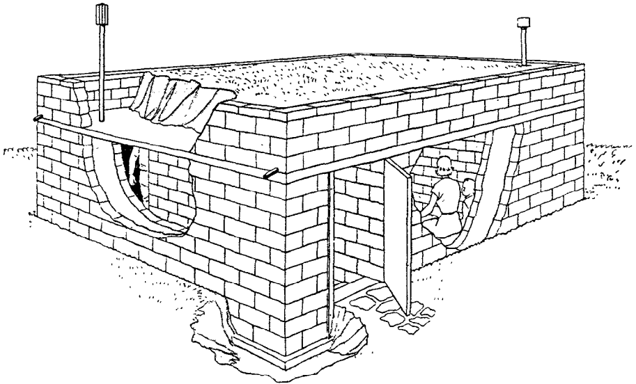
Figure 9.—Aboveground double-wall shelter
