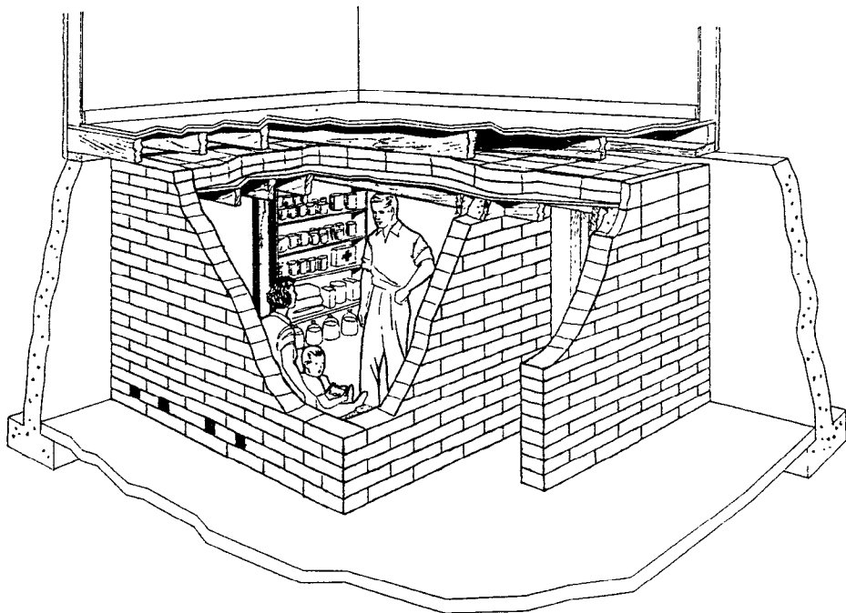
Figure 7—Basement Concrete Block Shelter
