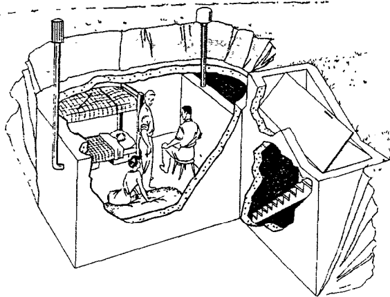
Figure 12.—Concrete basement shelter in new housing
