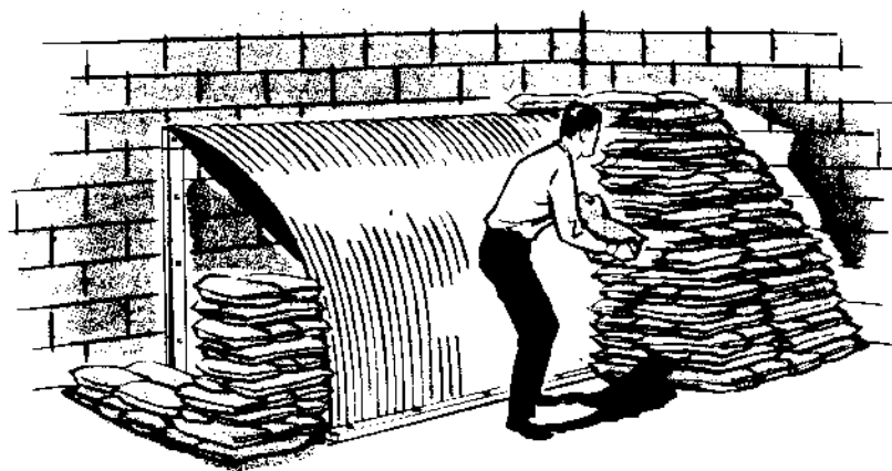
This four-person basement-corner shelter is made of curved asbestos-cement sheets which are covered with sandbags. Materials cost about $125.
