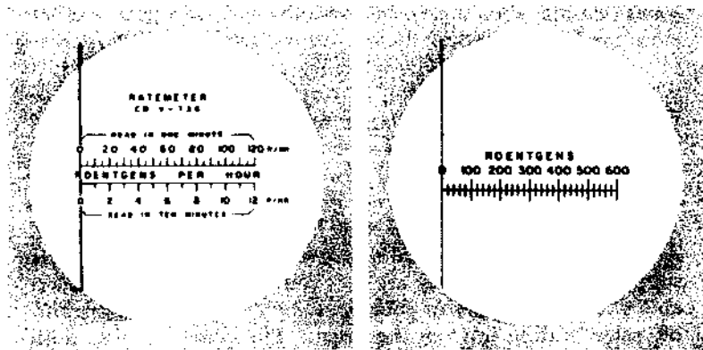
Enlarged view of a ratemeter scale. This particular model must be exposed to radiation for certain specific times to measure the dose rate (intensity) of radiation.
