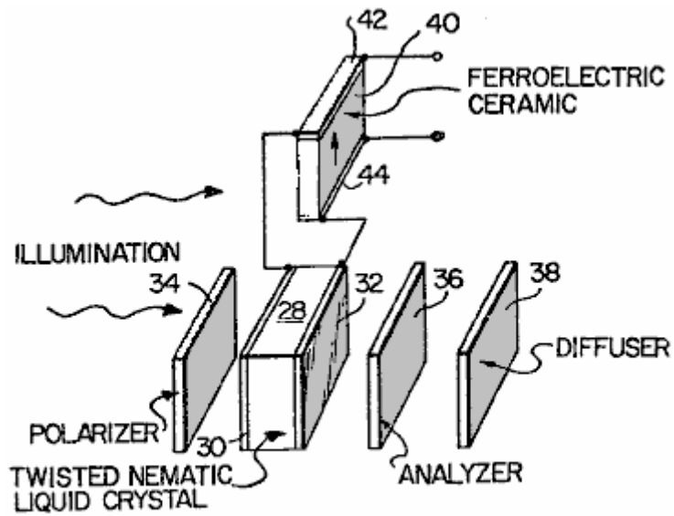
Fig.27 is a schematic illustration of an optical display apparatus utilising a ferroelectric ceramic material in accordance with the general teachings of the instant invention;
