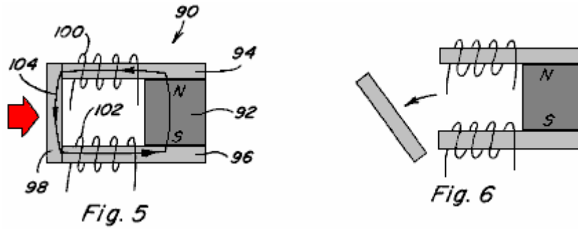
Fig.5 and Fig.6 are side views of a permanent magnet device including a permanent magnet having pole pieces positioned against the pole faces thereof and including a movable armature;
